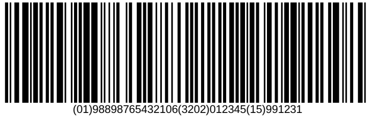
Figure 66: zint -b GS1_128 --compliantheight -d "[01]98898765432106[3202]012345[15]991231"
