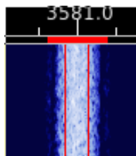
Figure 33.4 QPSK63 signal transmitting text data - waterfall view
