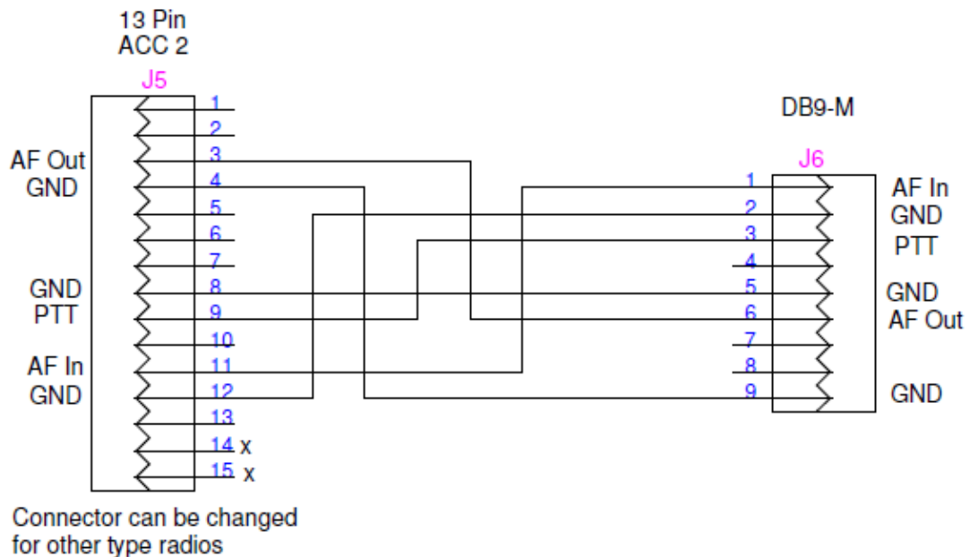
Figure 61.2 TS-2000 ACC-2 to DB9 Adapter
