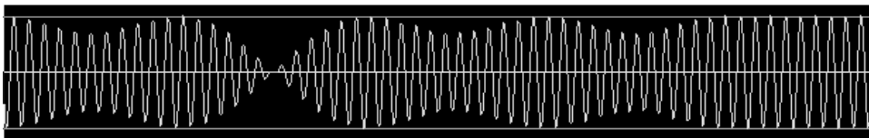
Figure 33.3 QPSK63 signal transmitting text data - oscilloscope - waterfall view
