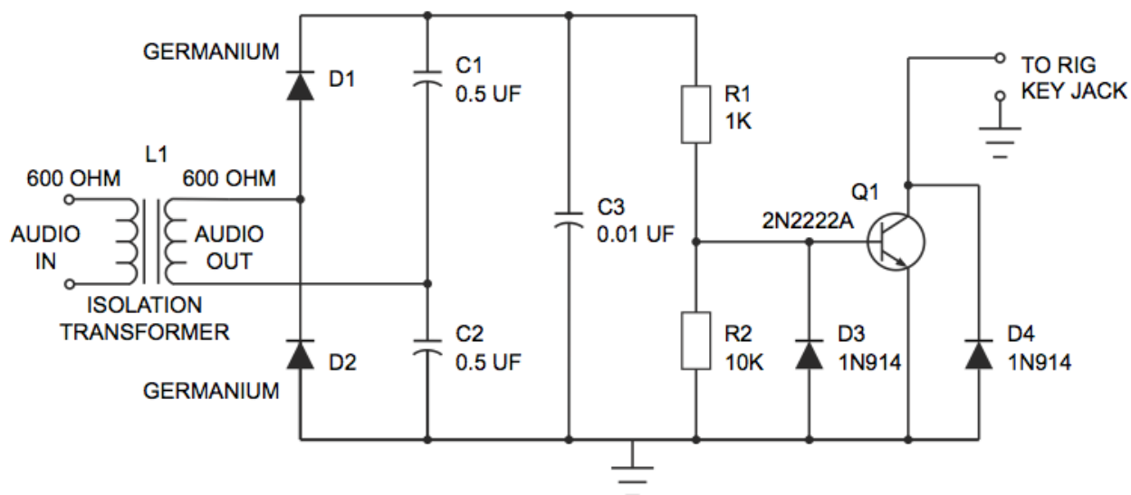
Figure 59.2 CW Keying Circuit
