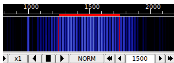
Figure 33.10 8PSK500F idle signal with pilot
