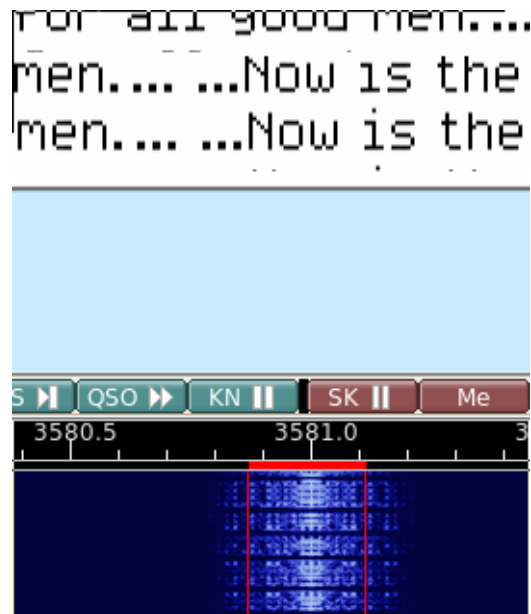
Figure 26.1 Feld-Hell, Slow Hell, Feld-Hell X5, and Feld-Hell X9 are all pulse
