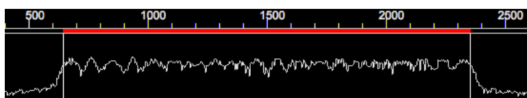
Figure 33.6 PSK63R20C signal transmitting text data - oscilloscope view
