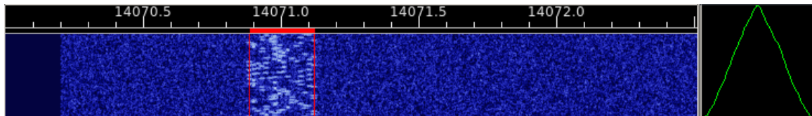
Figure 28.1 MFSK16 signal
