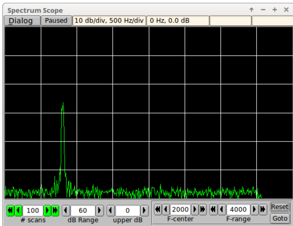
Figure 40.1 Spectrum Scope Display
