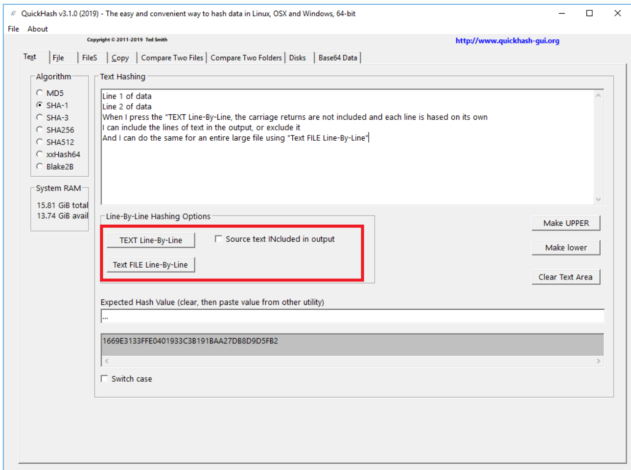
Illustration 3: The text hashing functions available since v2.6.7
