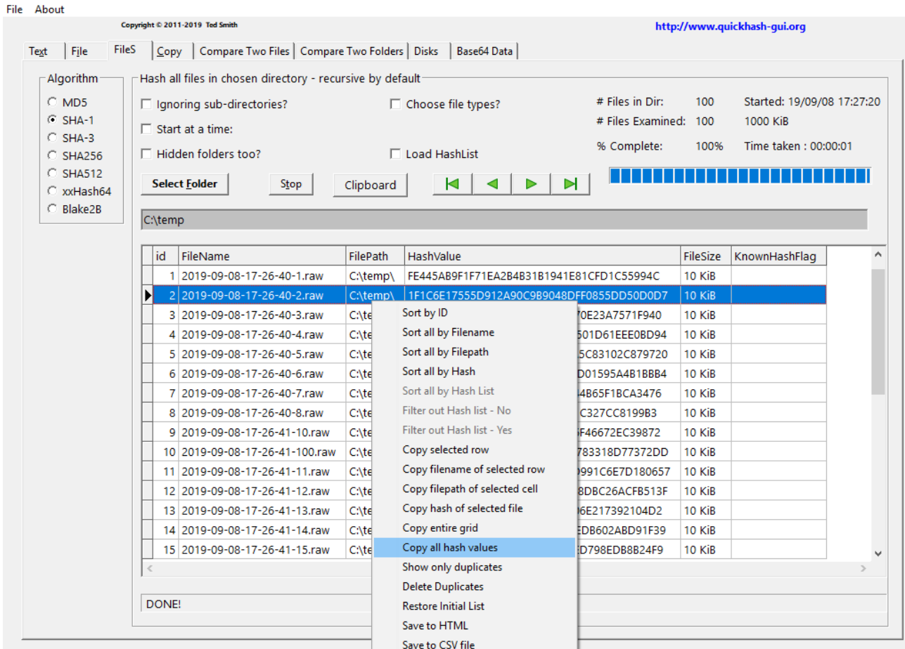
Illustration 7: Files hashed in FileS tab
