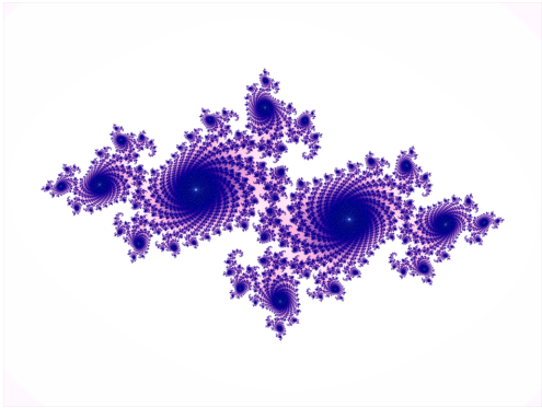
(a) 茉莉亚集分形
